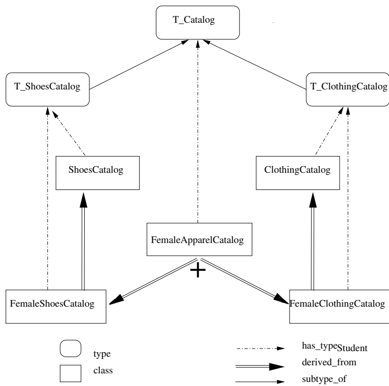
Figure 8: An Example of a Composed Derived Image Class
