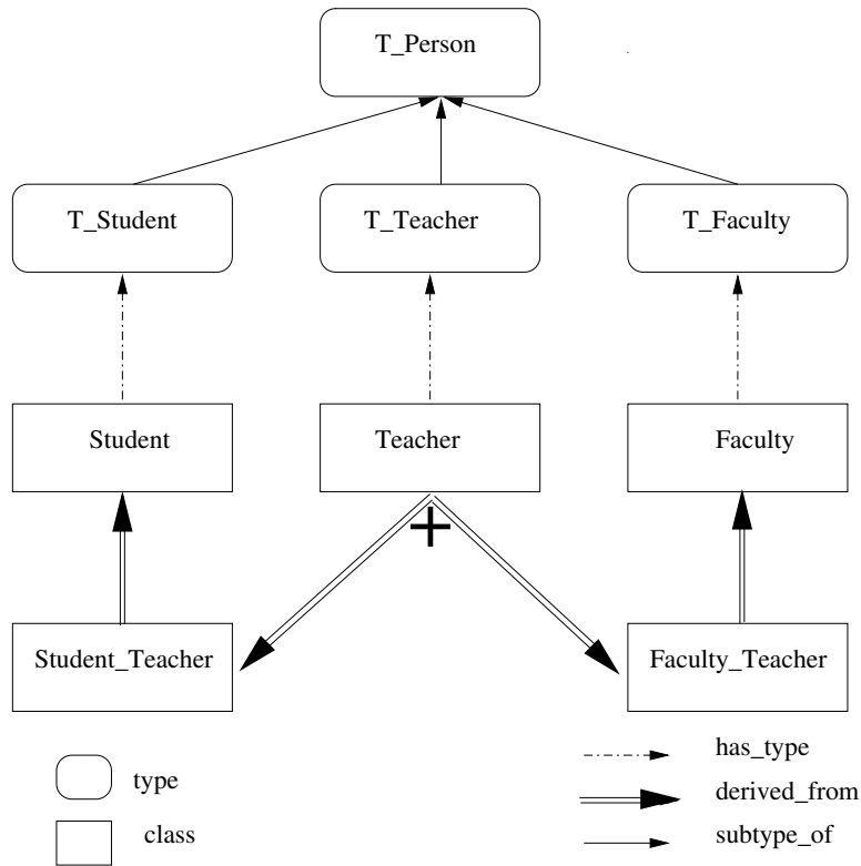
Figure 7: An Example of a Composed Derived Class and its Type.
