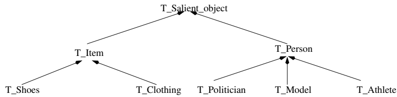
Figure 4: An Example of Logical Salient Object Hierarchy.
