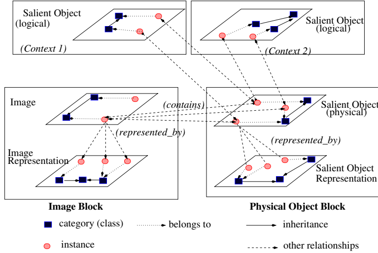
Figure 5: Image Views in DISIMA.
