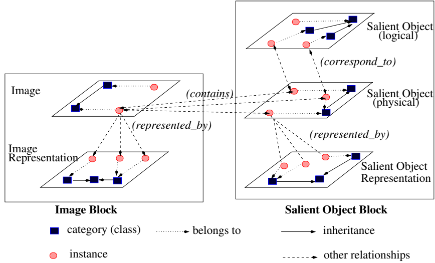
Figure 2: The DISIMA Model Overview.
