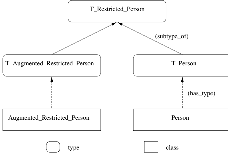
Figure 6: An Example of a Derived Class and its Type
