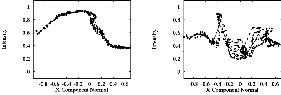
Figure 7. The joint distribution of data from the aligned and misaligned case above (left: aligned, right: misaligned). The weighted neighbor function approximation is shown as a thin black line.
