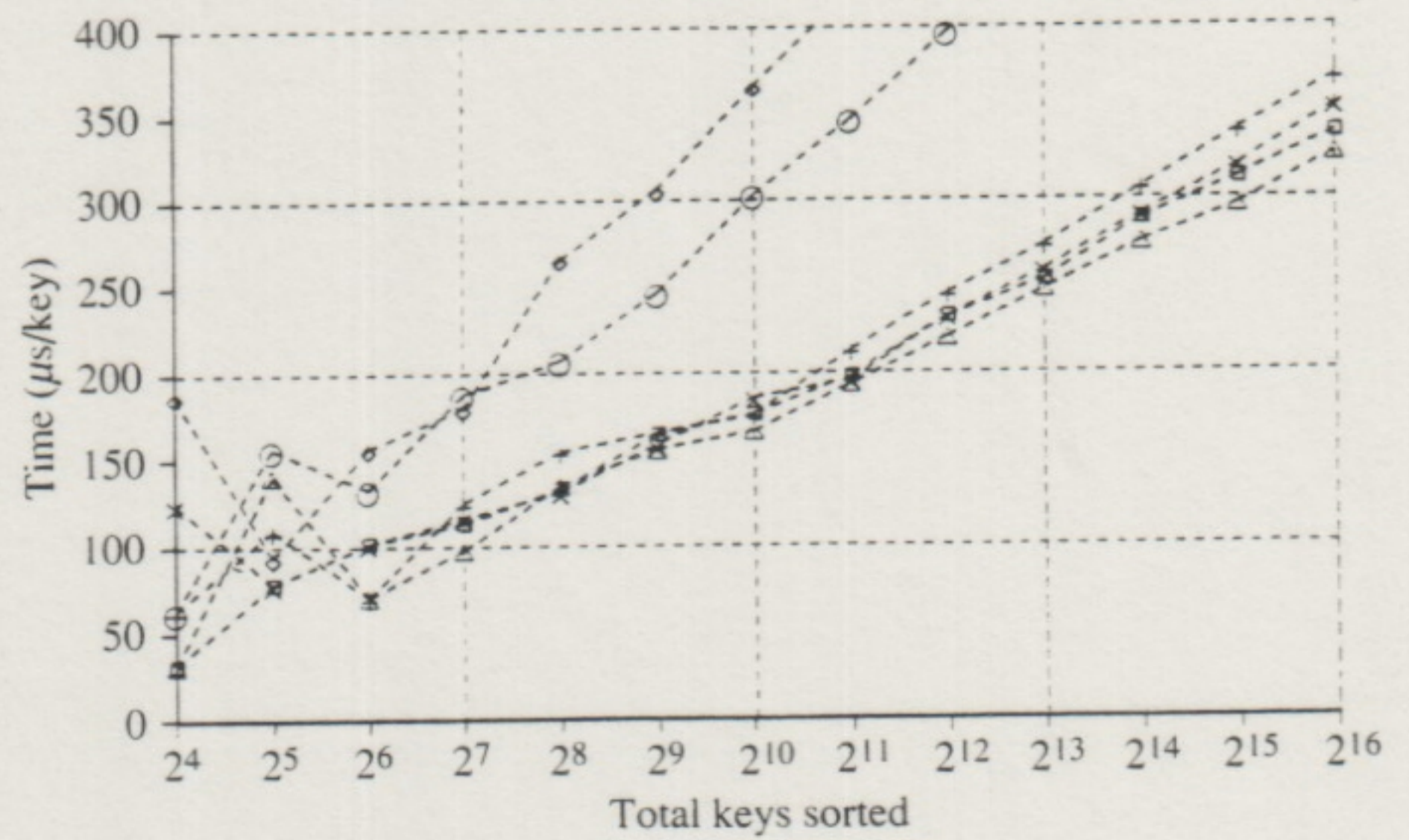
Figure 9. Time to Quicksort a 16-byte key.
