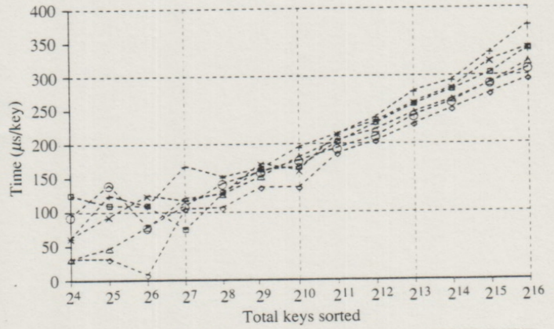
Figure 7. Time to Quicksort a 4-byte key.
