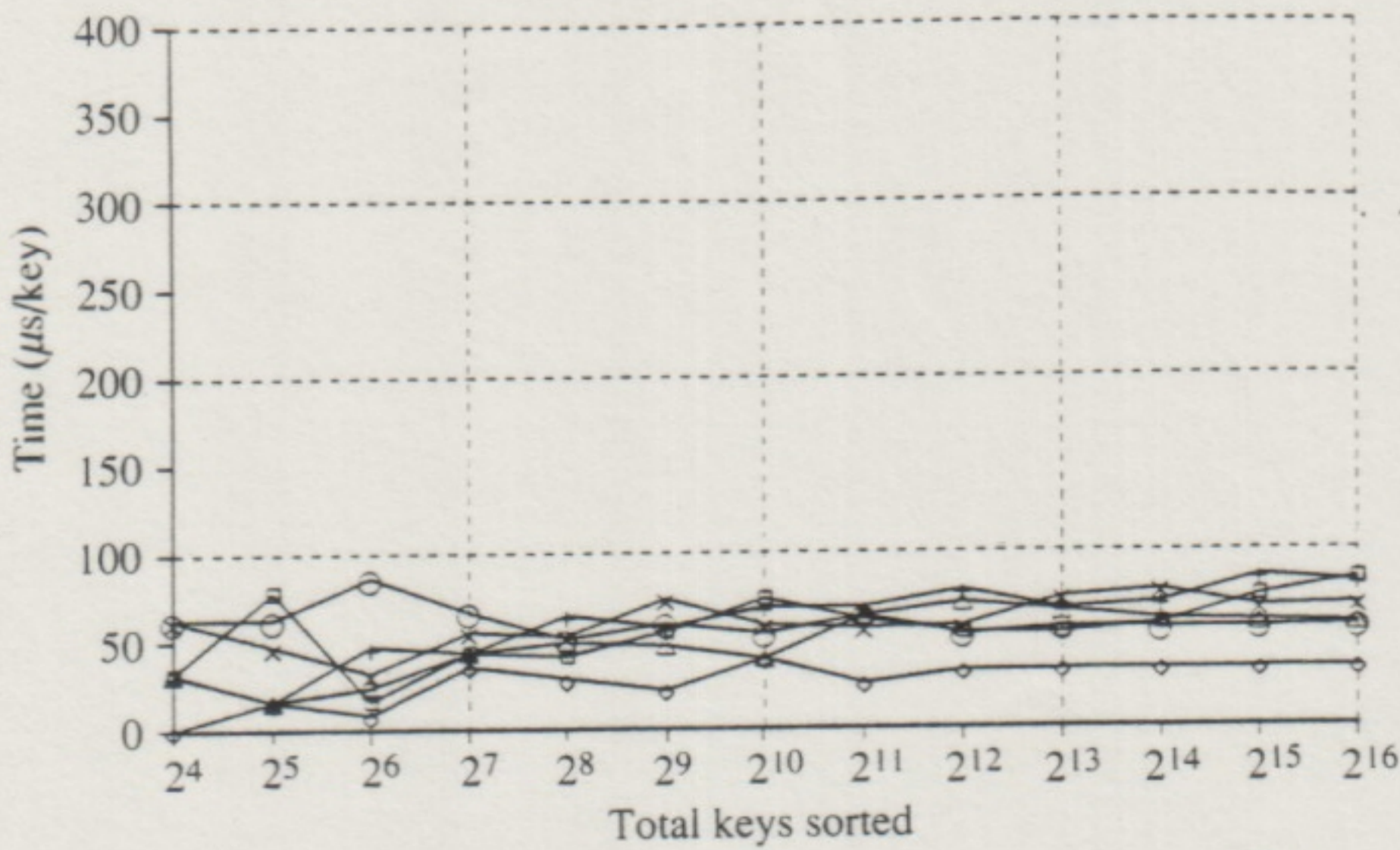
Figure 6. Time to radix sort a 4-byte key.
