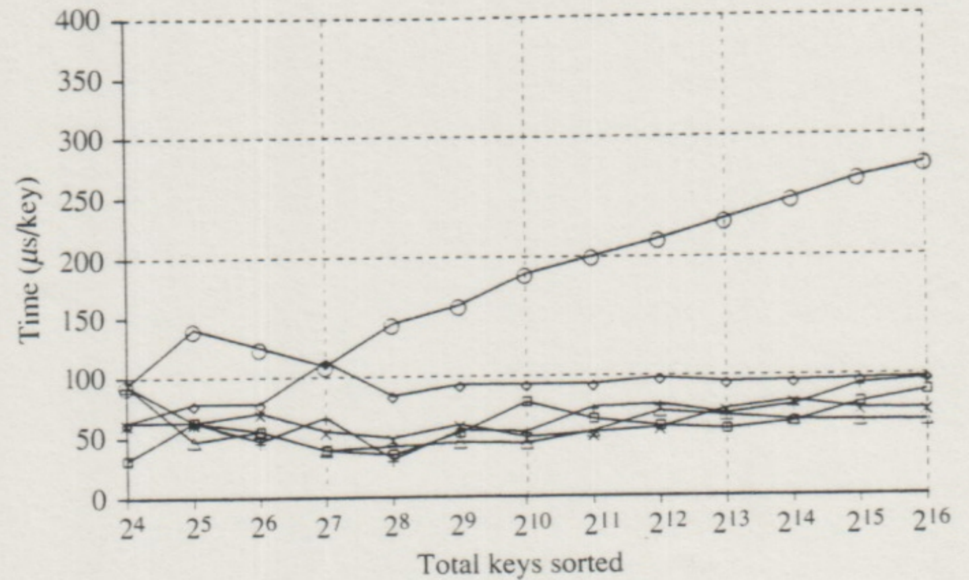
Figure 8. Time to radix sort a 16-byte key.
