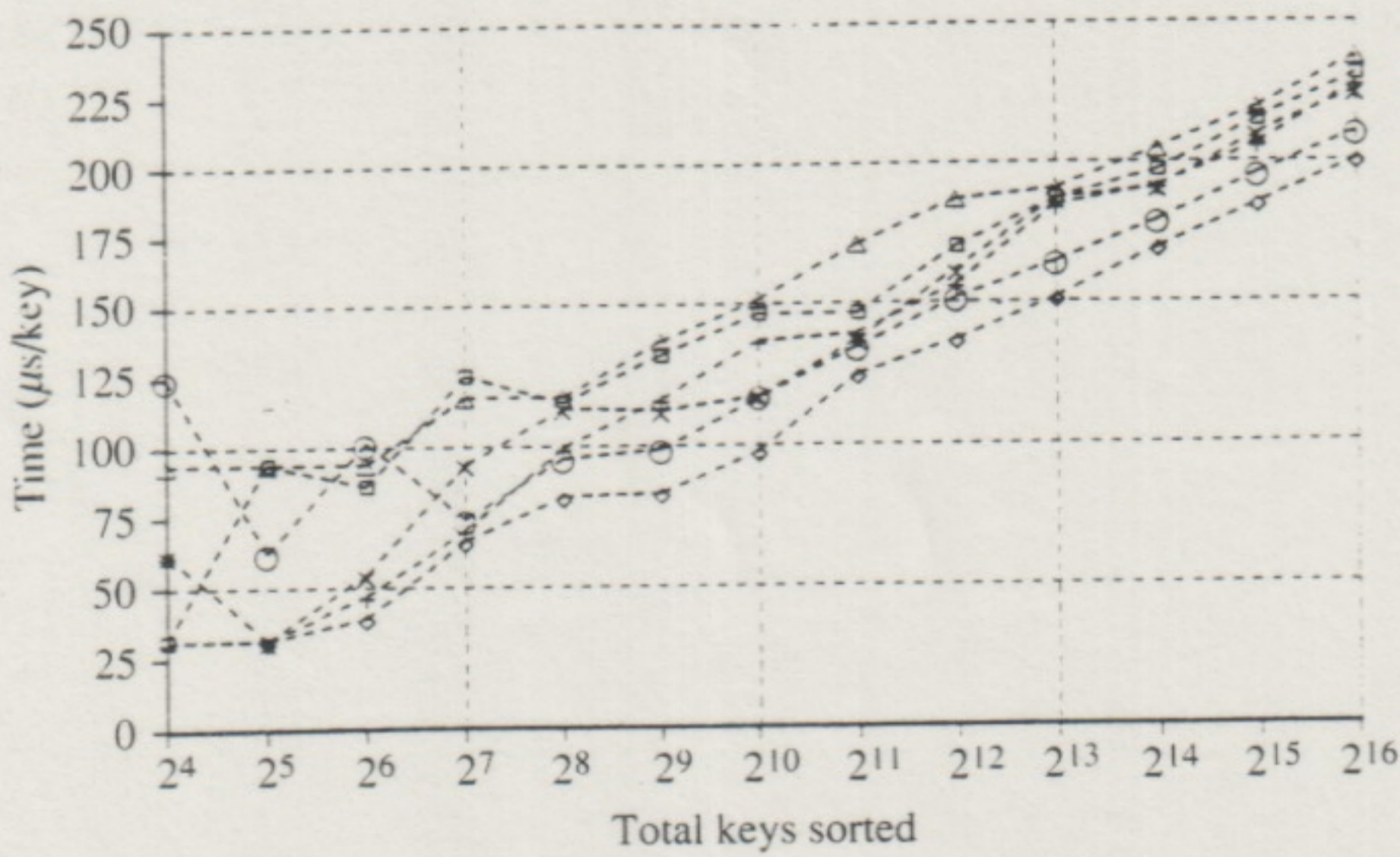
Figure 5. Time to Quicksort a 1-byte key.
