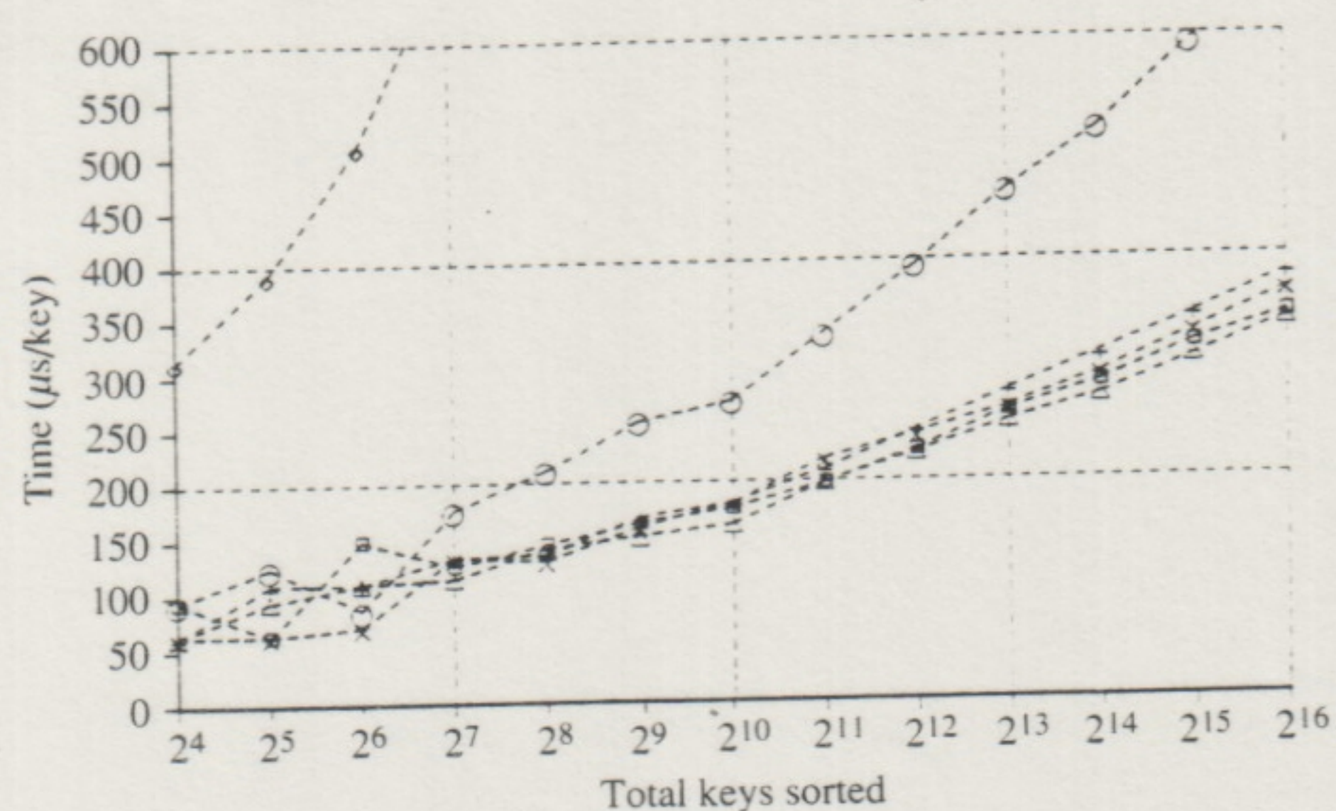
Figure 11. Time to Quicksort a 64-byte key.
