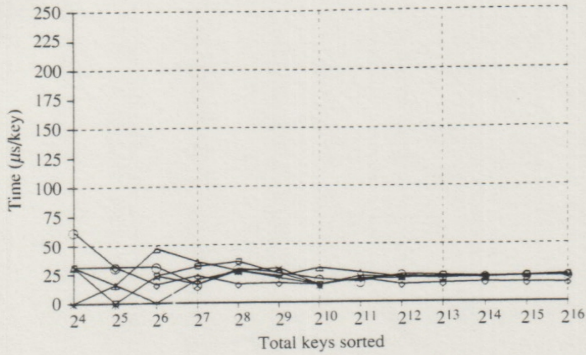
Figure 4. Time to radix sort a 1-byte key. Explanation of markings for Figs 4-11: \diamond --- \diamond , all keys same; \circ --- \circ , 2 symbols; +---+, 16 symbols; \times --- \times , 32 symbols; \square --- \square , 64 symbols; \triangle --- \triangle , 256 symbols (all).
