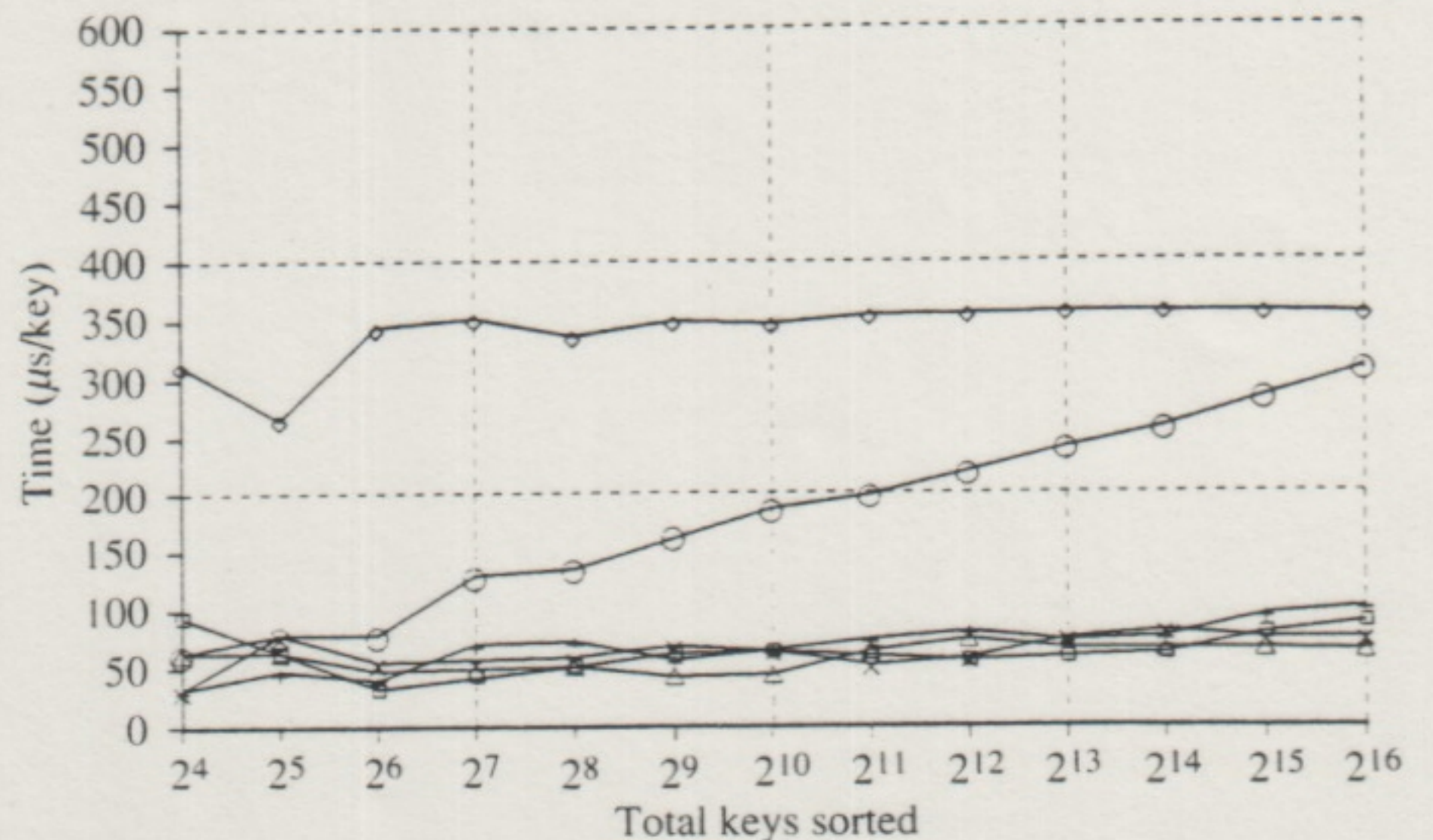
Figure 10. Time to radix sort a 64-byte key.
