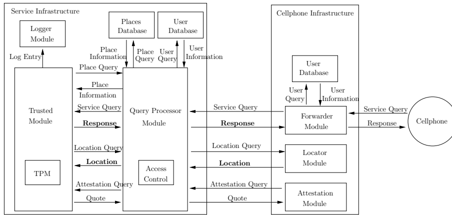
Figure 1: Architecture for location-based services. A cellphone sends a service query via the cellphone infrastructure to the service infrastructure, which uses the Trusted Module for processing the query and generating a response. Items in bold are encrypted (Response and Location).
