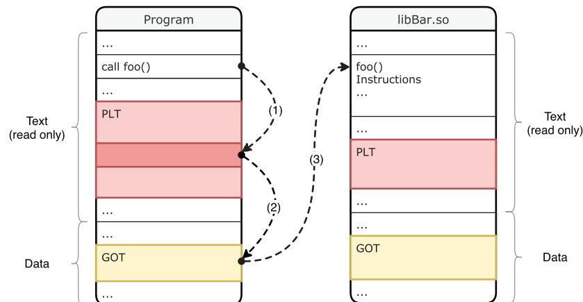
Fig. 9. Execution flow for call to external function foo , adapted from Reference [34].
