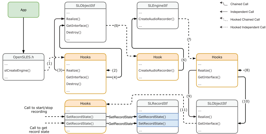
Fig. 5. Hook flow of OpenSL ES.
