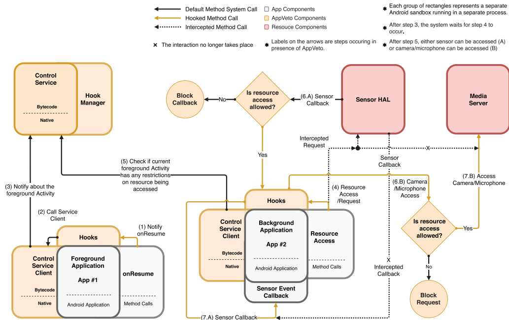
Fig. 6. AppVeto overview.
