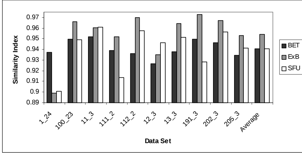
Figure 4: Similarity index for the different segmentation algorithms. Holes not filled.
