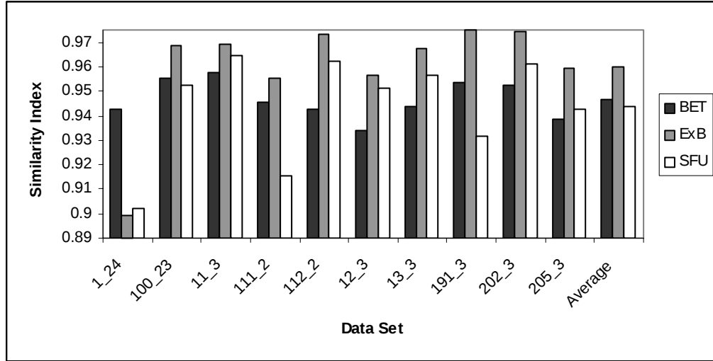
Figure 5: Similarity index for the different segmentation algorithms. Holes filled.
