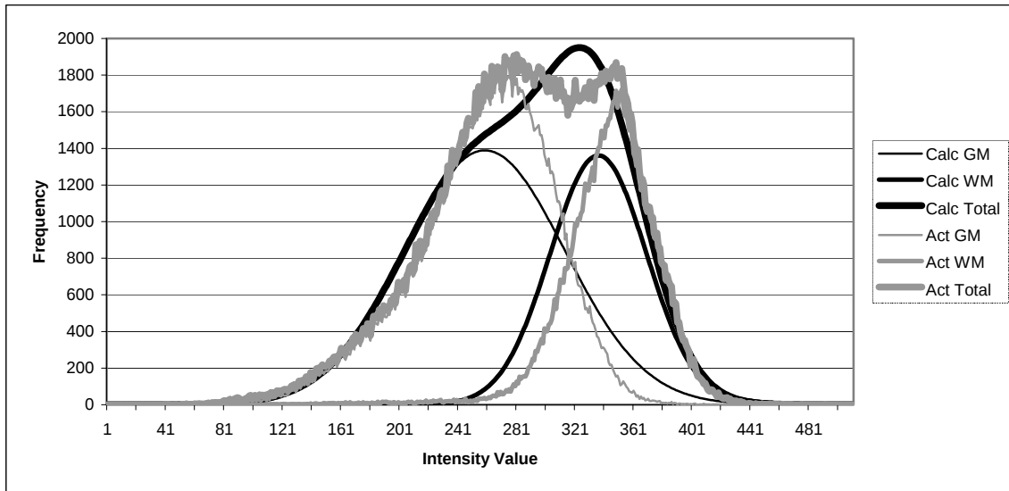
Figure 6: Histogram for dataset 1_24 under the brain mask
