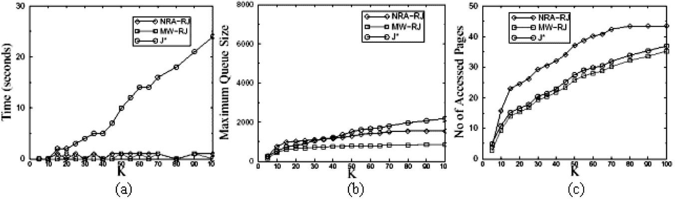
Fig. 5. Performance comparison for NRA-RJ, J^* , and MW-RJ for m = 3
